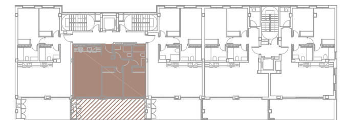
FLOOR 2
