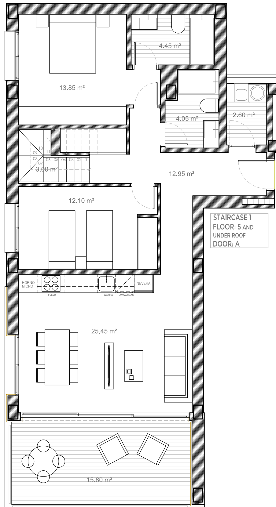
FLOOR 5
